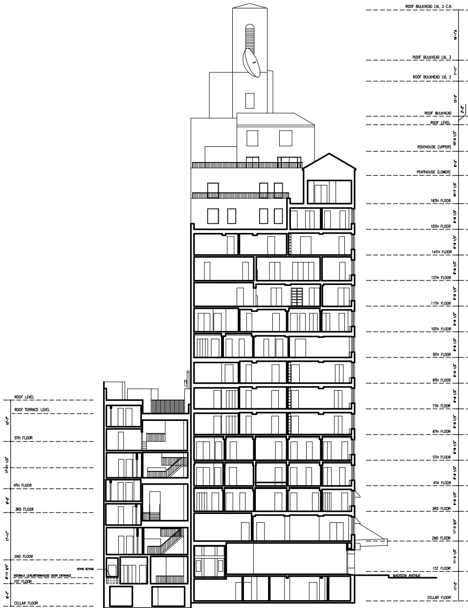
SECTION 1-1
