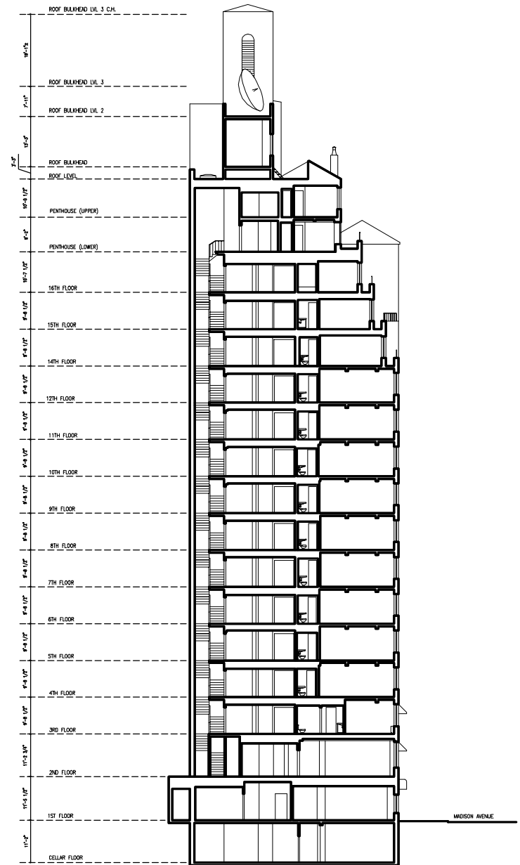
SECTION 2-2
