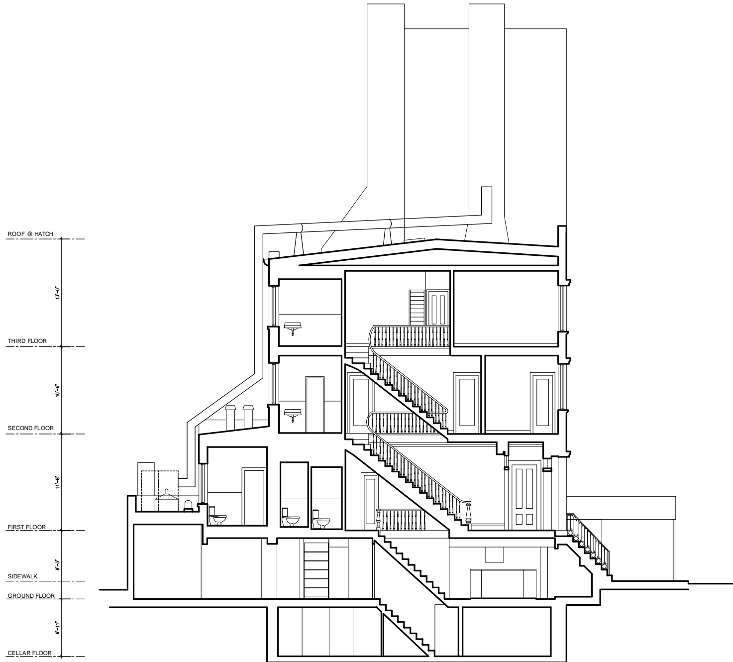
Residential Cross Section New York, NY
